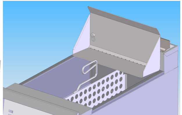
TANK DIVIDER OPTION AND CRUMB TRAY ACCESSORY
